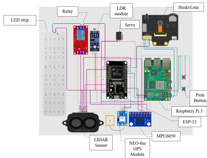
Fig. 5 Circuit Schematics on Cirkuit Designer
